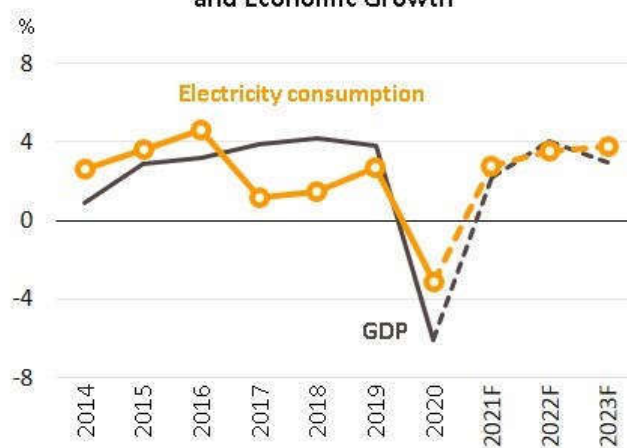
Figure 12: Trend of Electricity Demand and Economic Growth
